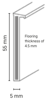
D 60 (without sealing lip)
