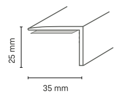
Self-adhesive variant (on request)
